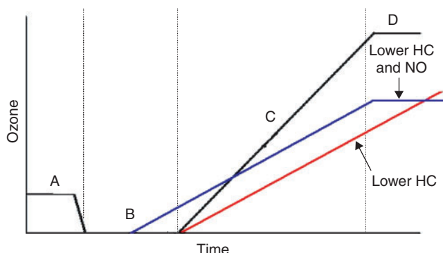
Fig. 1. Schematic cross-section of ozone formation. Wind is assumed to blow at a fixed rate from (A) to (D); time and distance are equivalent. The sections are (A) upwind, (B) central urban area, (C) downwind, (D) further downwind, not often reached because of sunset.
